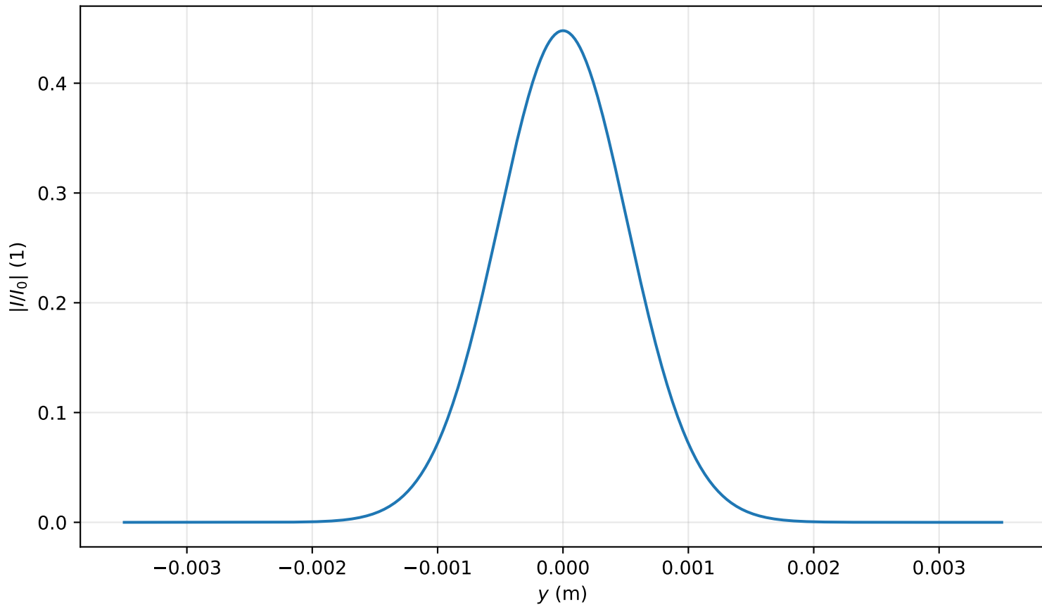
Intensity profile I(x = 0, y, z = 2.388)/I_0 , P_{in}=0.1P_{cr} , artificial time
